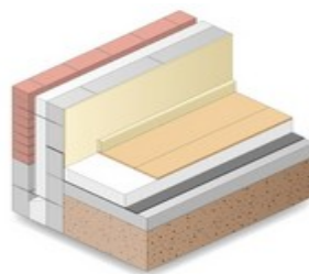
Floating Floor
