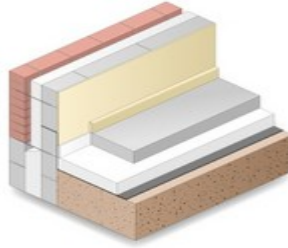
Below Concrete Slab
