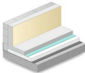
Cold Store Flooring in EPS or XPS
