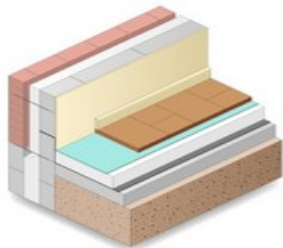
Above Concrete Slab
