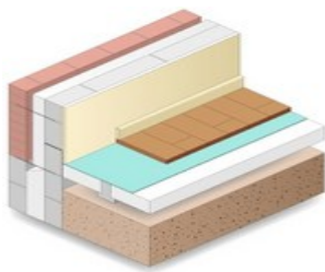
Concrete Suspended Floor
